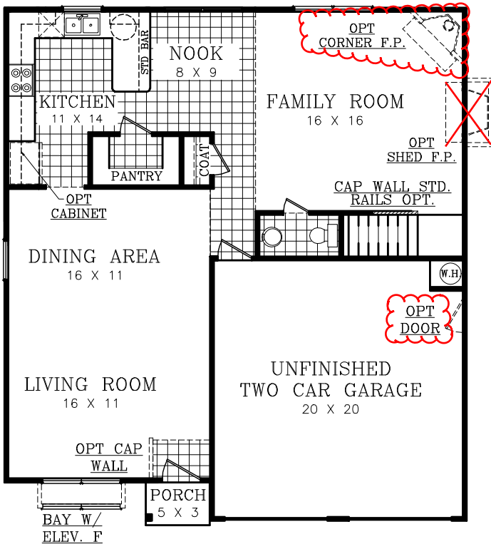
1st Floor Elevation A & F
